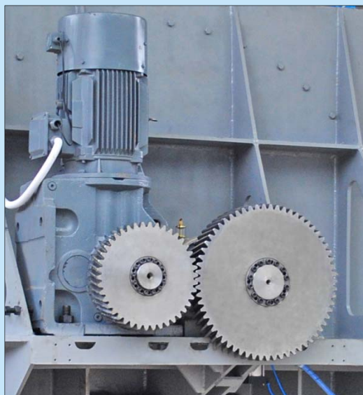
Wassar 360/550 齒輪驅動系統 Gear driving system of Wassar 360/550
