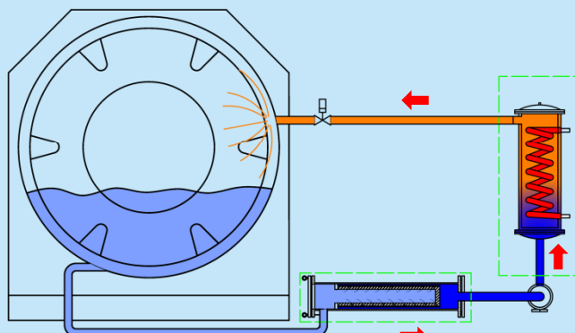
外置式間接加熱系統示意圖 Diagram of External indirect heating system
