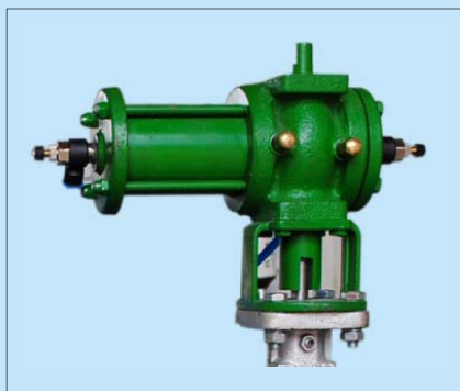
O-I-04-3-1 電控氣動入水系統 - Ø3" Electric Controlled Pneumatic Water Feeding System - Ø3"
